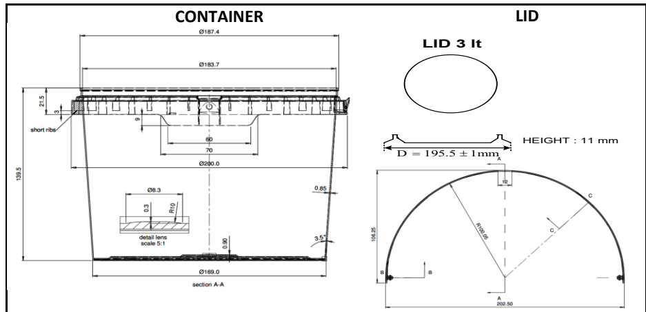
PRODUCT DRAWING & LIDS
