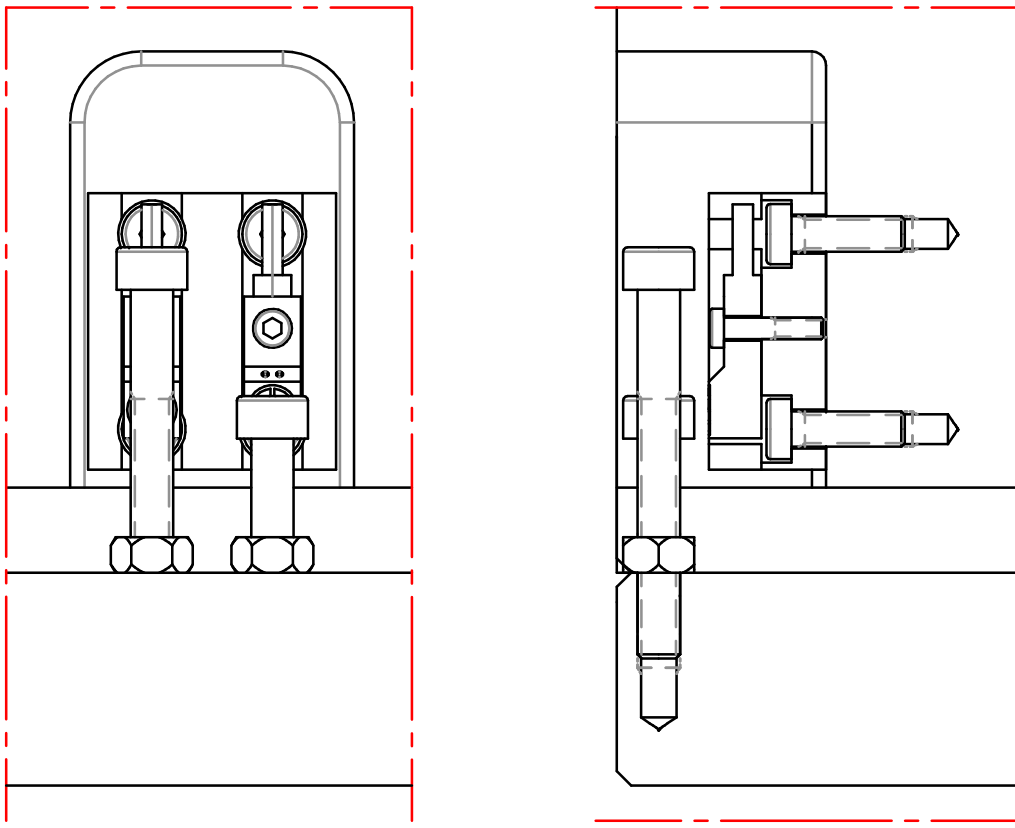
Sensor Omron E2S-W21 Non operator side
