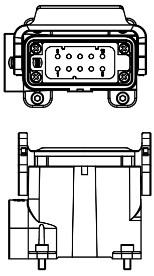
PLUGHOUSING for detection sensors ejectionplate with HARTING connector: (on top / non operator side)
