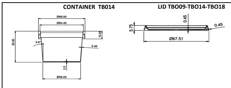
PRODUCT DRAWING & LIDS
