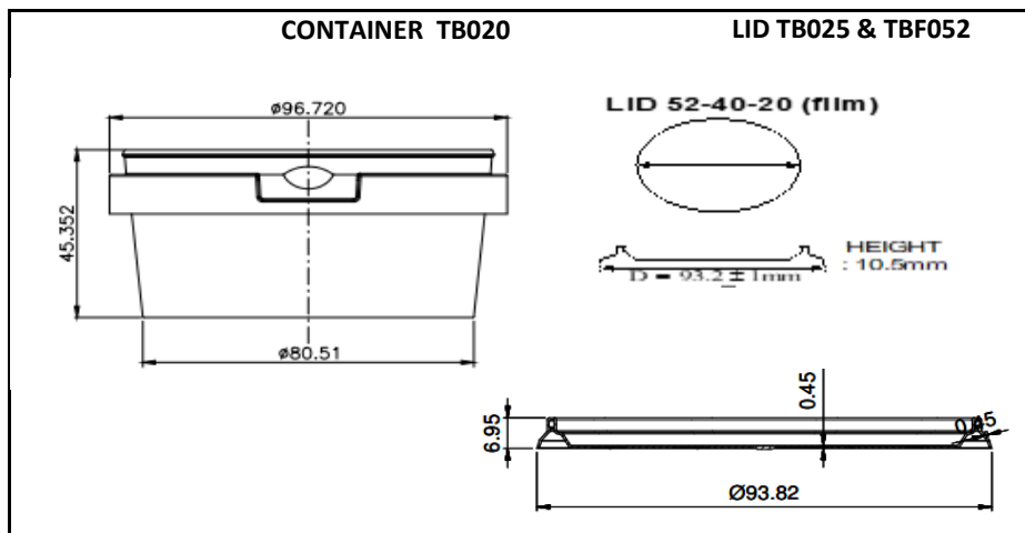
PRODUCT DRAWING & LIDS
