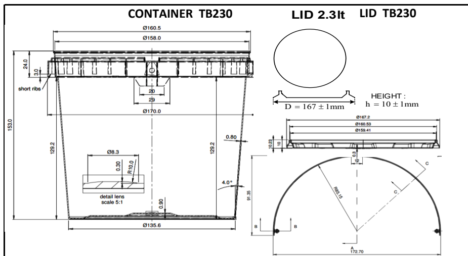
PRODUCT DRAWING & LIDS
