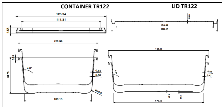
PRODUCT DRAWING & LIDS
