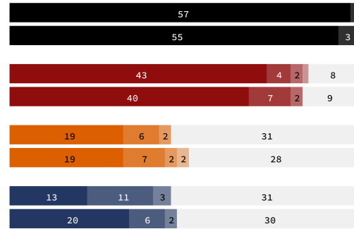
Figure 2.16: Red-Black Trees
