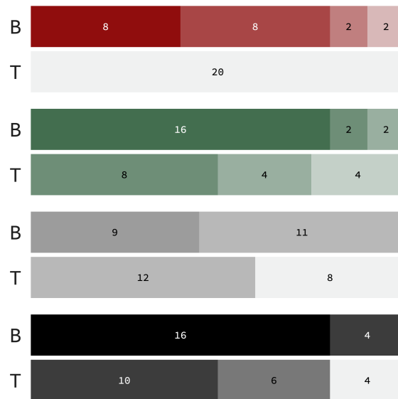
(c) STL
