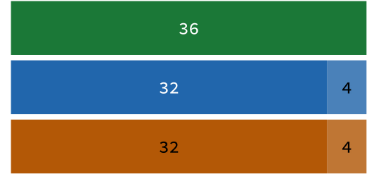
(b) Correct-by-construction
