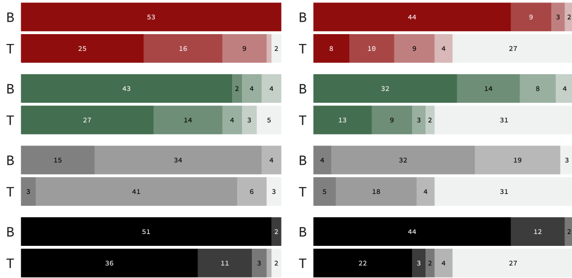
(a) BST
