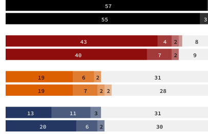
Fig. 17. Red-Black Trees
