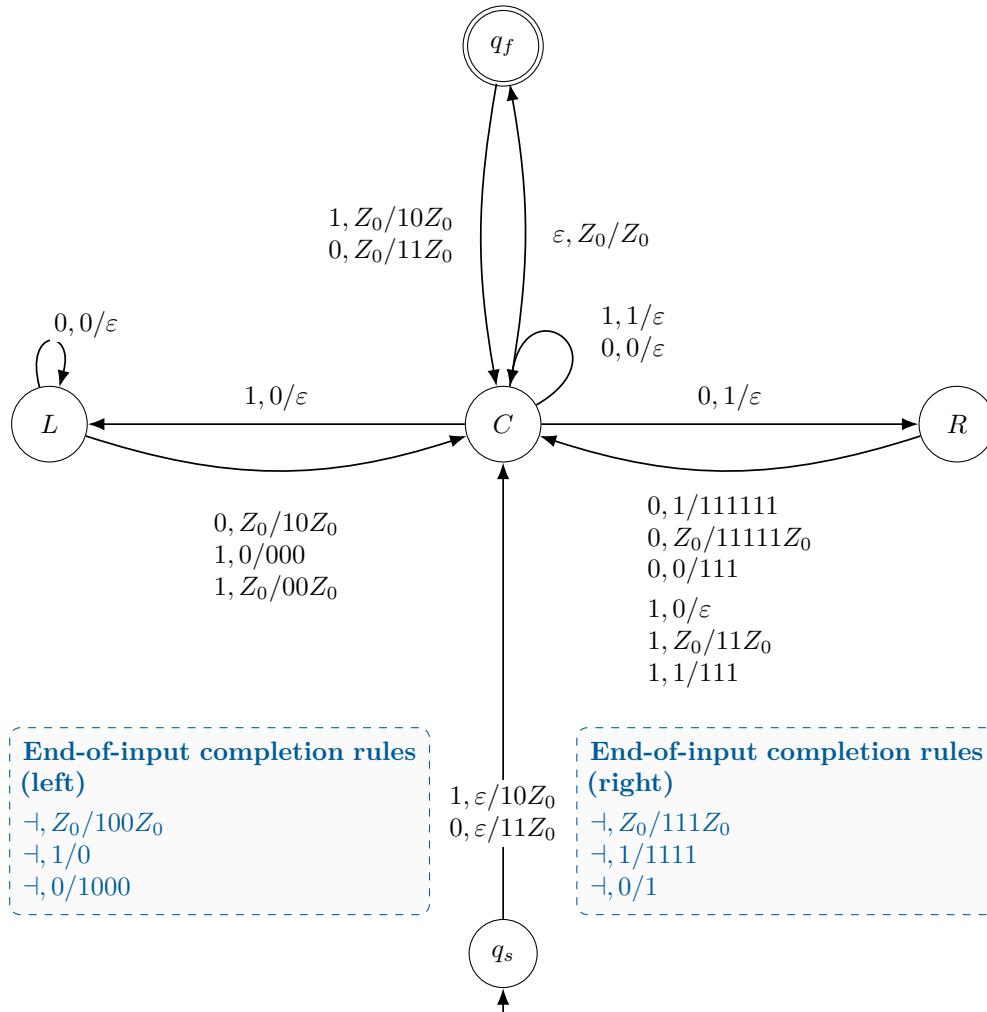
Figure 87.1: The empty-input-excluded original DPDA revisited after the general theory. This is the same formalized machine as Figure 1.1, deliberately repeated so that the final interpretation can be read against the original object.
