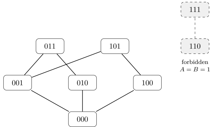
Figure 43.1: Hasse diagram of the six admissible 2:1 schedules. The schedule bits are ordered by inclusion of eager sites A, B, C . The two omitted cube vertices 110 and 111 are shown separately as forbidden because A and B cannot be simultaneously eager.
