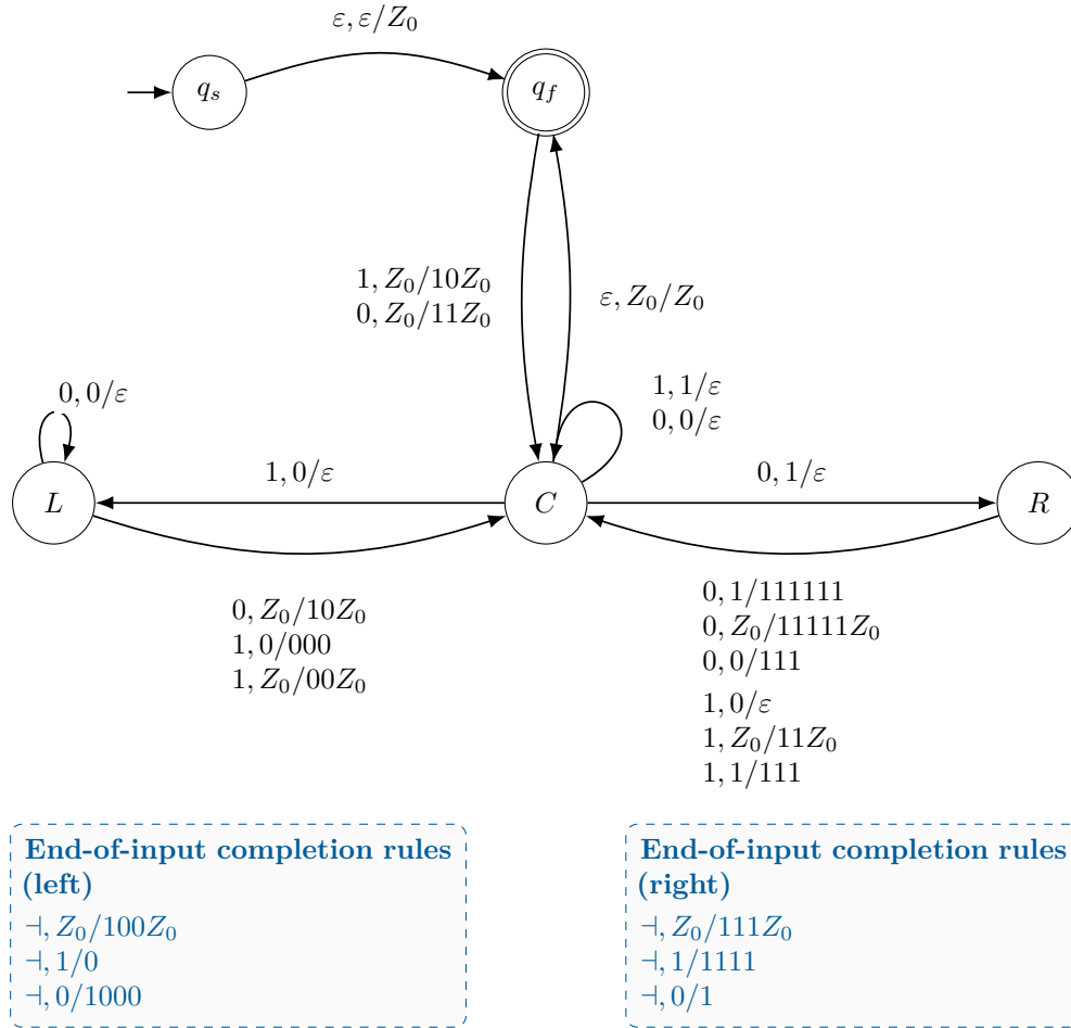
Figure 87.2: The empty-input-included original DPDA revisited. This is the same recognition/completion core as Figure 1.2; the wrapper accepts \varepsilon .
