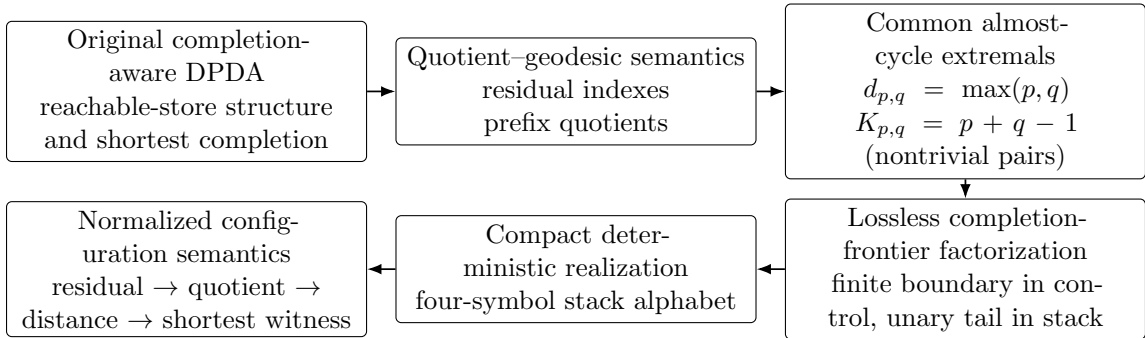
Figure 1: The six main results as one structural chain. The completion-aware stack semantics leads to quotient geometry and common almost-cycle extremals; the exact frontier then supports lossless factorization, compact realization, and configuration-level decoding.
