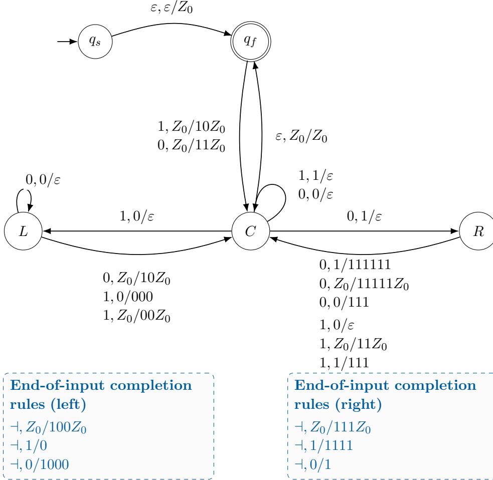
Figure 3: Formalized redrawing of the original 2:1 DPDA variant with the empty input included. The center/left/right recognition logic and the dashed end-of-input completion callouts are the same as in figure 2; the initialization/final-state structure additionally accepts \epsilon . Hence this variant recognizes the standard language L_{2,1} , while the previous variant recognizes L_{2,1} \setminus \{\epsilon\} . The source design is archived at https://github.com/alperenbutun/dpda-ones-twice-zeros .
