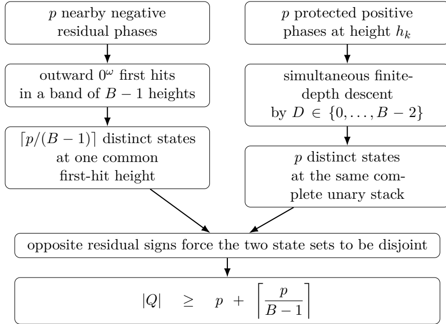
Figure 90.1: Architecture of the new unrestricted bounded-replacement lower bound for p \geq q . The bounded rewrite length is used only to create the finite first-hit band; all representation freedom before that crossing is absorbed by residual rigidity and protected finite-depth descent.
