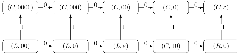
Figure 3.1: Exact configuration ladder for k = 2 . The upper boundary is canonical completion; the lower boundary postpones the unique required 1 as long as possible.
