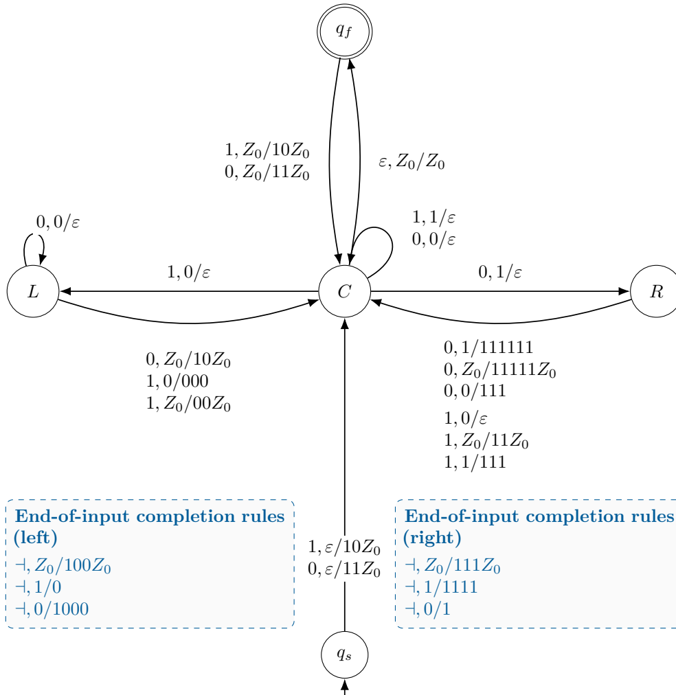
Figure 114.1: The empty-input-excluded original DPDA revisited after the general theory. This is the same formalized machine as Figure 1.1, deliberately repeated so that the final interpretation can be read against the original object.
