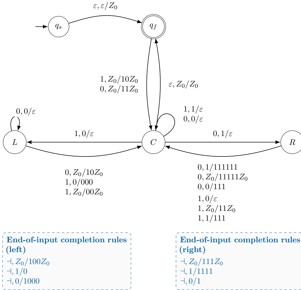
Figure 114.2: The empty-input-included original DPDA revisited. This is the same recognition/completion core as Figure 1.2; the wrapper accepts \varepsilon .
