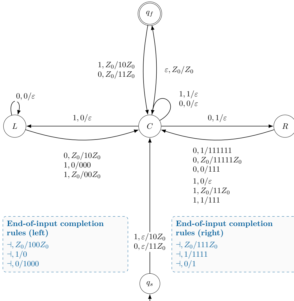
Figure 83.1: The empty-input-excluded original DPDA revisited after the general theory. This is the same formalized machine as Figure 1.1, deliberately repeated so that the final interpretation can be read against the original object.
