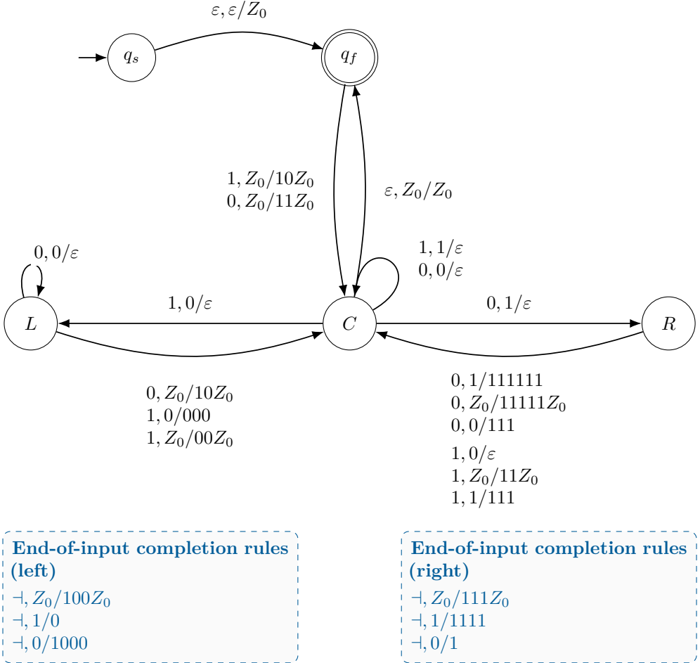
Figure 55.2: The empty-input-included original DPDA revisited. This is the same recognition/completion core as Figure 1.2; the wrapper accepts \varepsilon .
