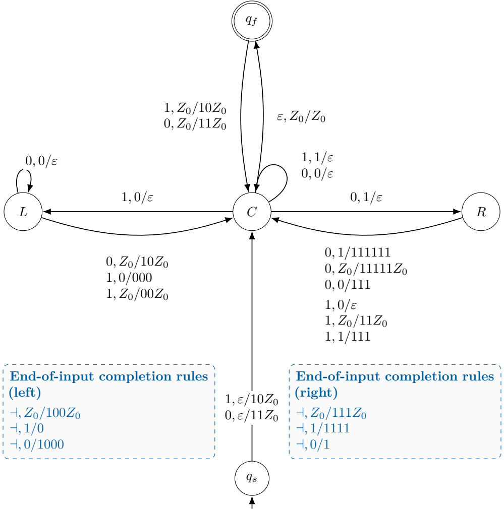
Figure 55.1: The empty-input-excluded original DPDA revisited after the general theory. This is the same formalized machine as Figure 1.1, deliberately repeated so that the final interpretation can be read against the original object.
