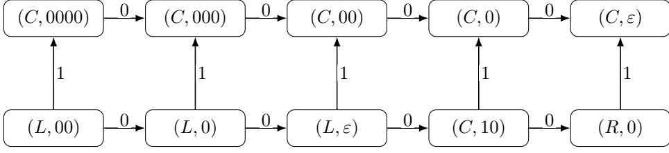
Figure 3.1: The exact configuration ladder for k = 2 . The source (L, 00) has residual 7 and minimum demand (4, 1) . Its five shortest continuations are 10000, 01000, 00100, 00010, 00001. The upper boundary is canonical completion; the lower boundary postpones the unique required 1 maximally.
