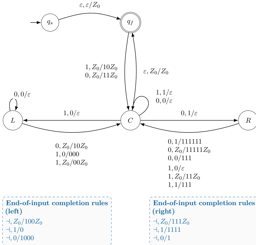
Figure 71.2: The empty-input-included original DPDA revisited. This is the same recognition/completion core as Figure 1.2; the wrapper accepts \varepsilon .
