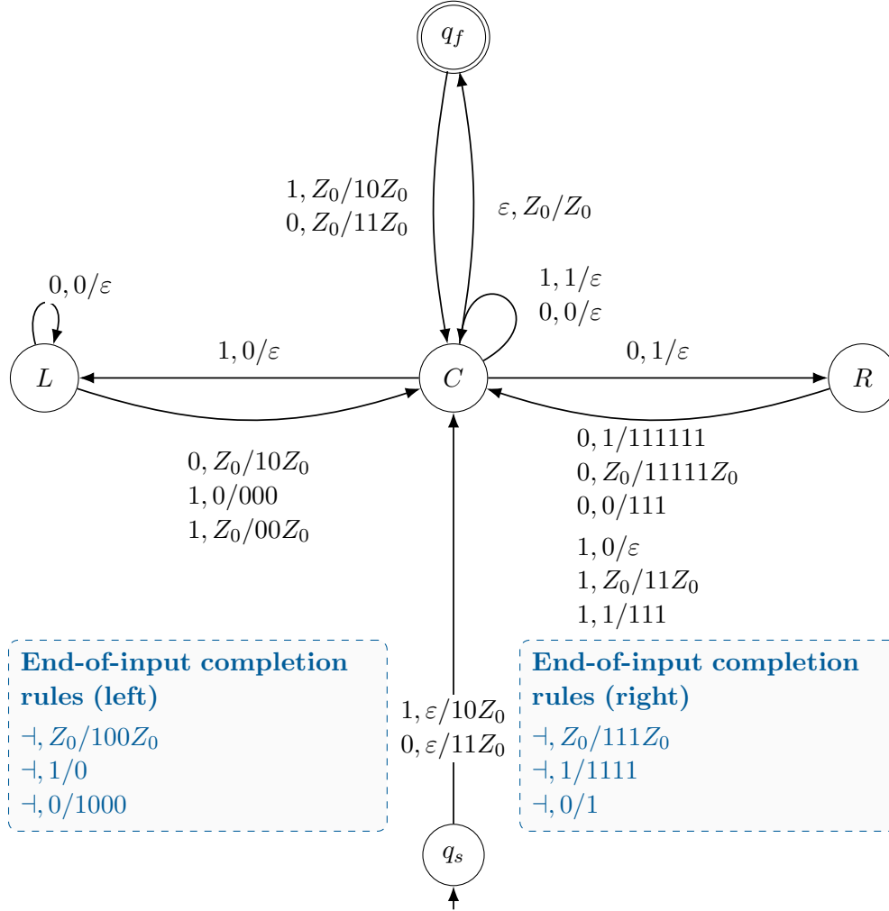
Figure 2: Formalized redrawing of the original 2:1 DPDA variant with the empty input excluded. Solid arrows are ordinary recognition transitions. Dashed callout boxes list the completion rules enabled only by the right endmarker \neg after the binary input has been exhausted; the same distinction remains visible in grayscale. The left-state rule \neg, 1/0 is retained for fidelity to the original completion list, but its source condition is unreachable because every reachable left-state stack belongs to 0^* . The source design is archived at https://github.com/alperenbutun/dpda-ones-double-zeros .
