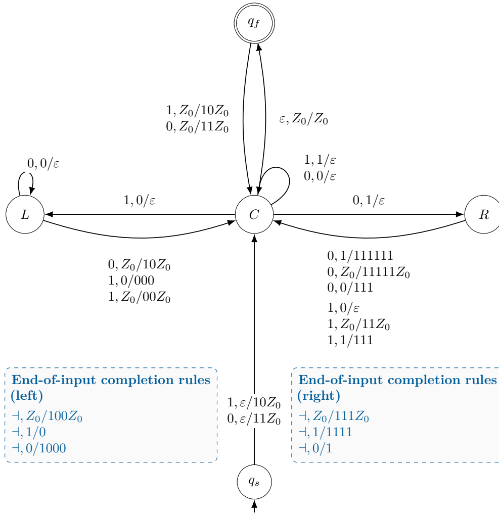
Figure 106.1: The empty-input-excluded original DPDA revisited after the general theory. This is the same formalized machine as Figure 1.1, deliberately repeated so that the final interpretation can be read against the original object.
