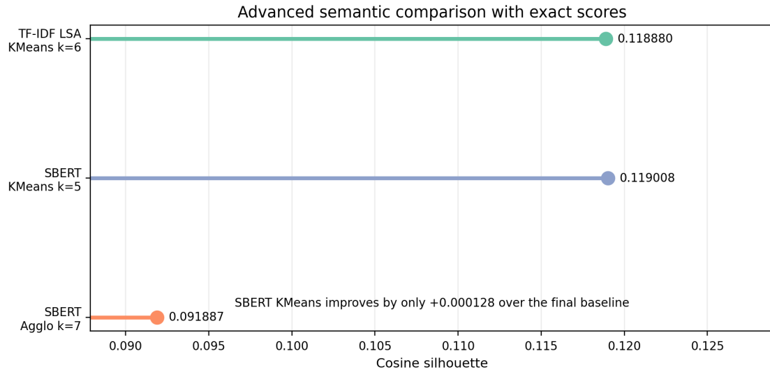
Figure 6: Advanced semantic comparison with exact scores. The first two scores look the same when rounded to three decimals, but they are not exactly equal.
