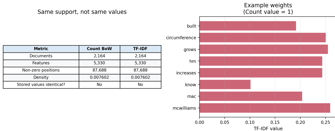
Figure 2: Count and TF-IDF use the same vocabulary support, but the stored values are different.
