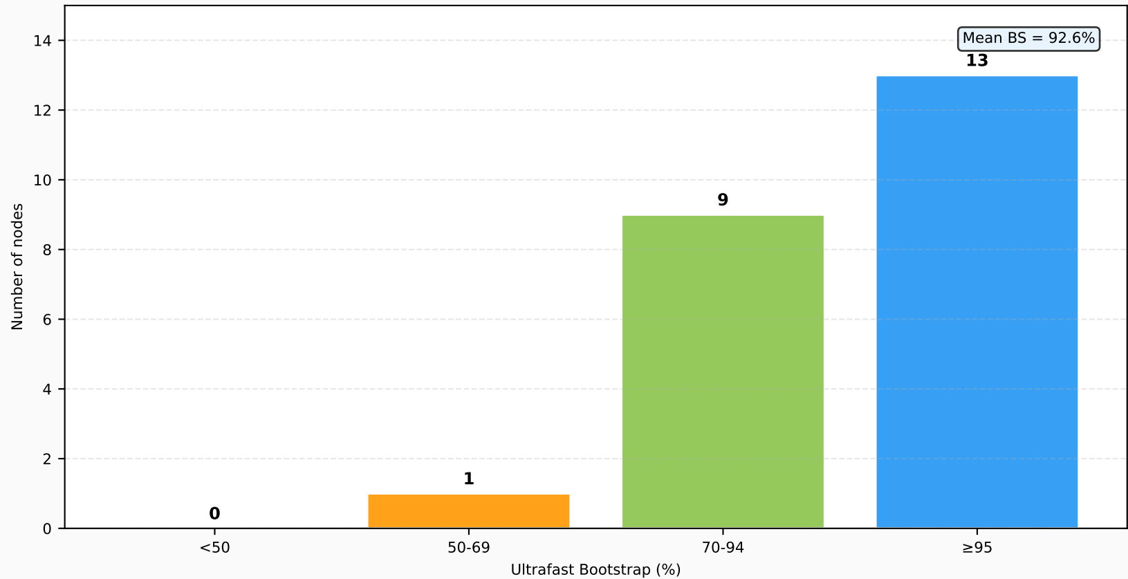
D Bootstrap Support Distribution (n=23 nodes)
