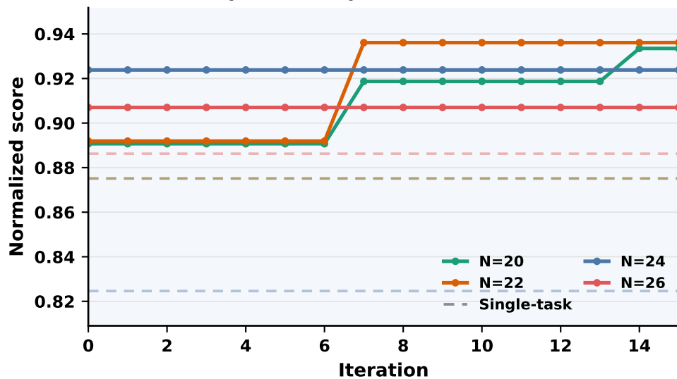
Task-Specific Adaptation Task Breakdown
