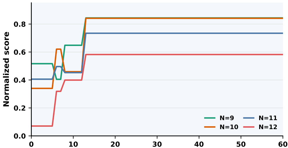
Task-Specific Adaptation Task Breakdown
