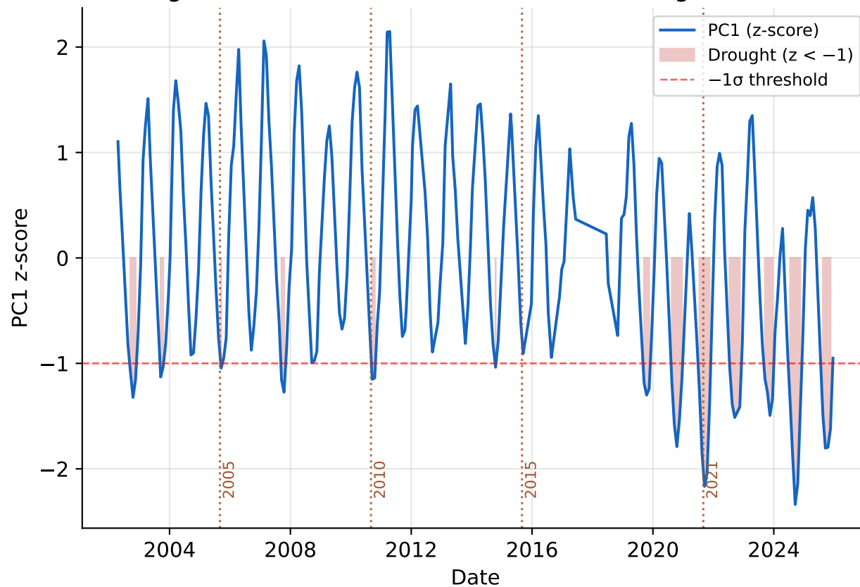
Figure 2b — PC1 Time Series (GRACE Drought Index)
