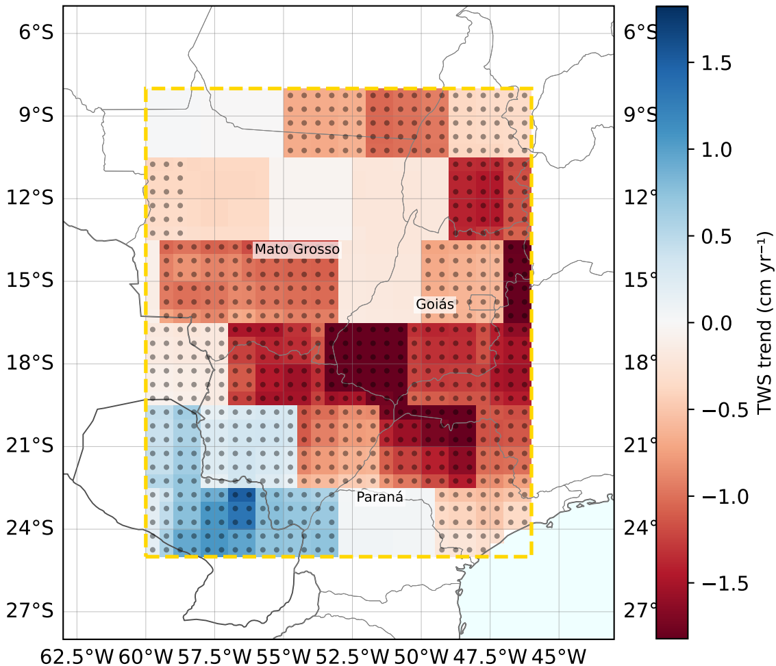
Stippling: p < 0.05 | Gold box: study region
