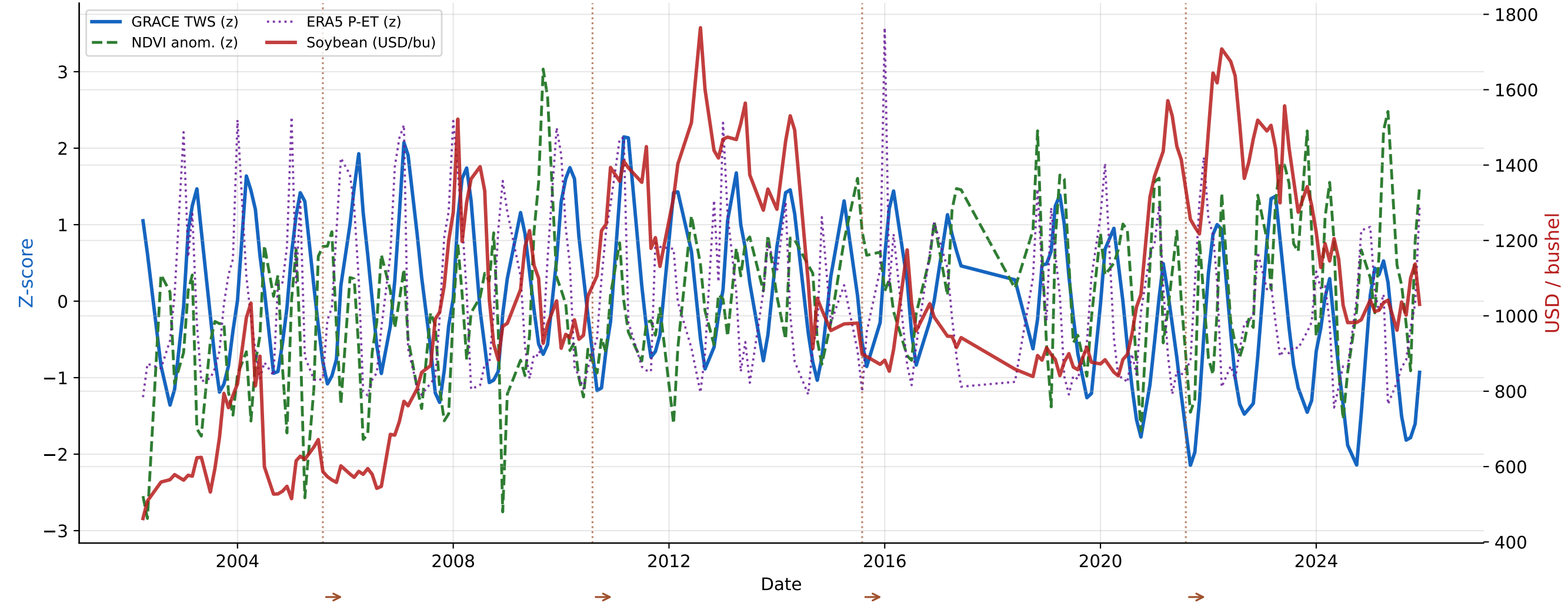
GRACE TWS · NDVI · P-ET · Soybean Futures Arrows: drought onset -> market reaction (~5 months)
