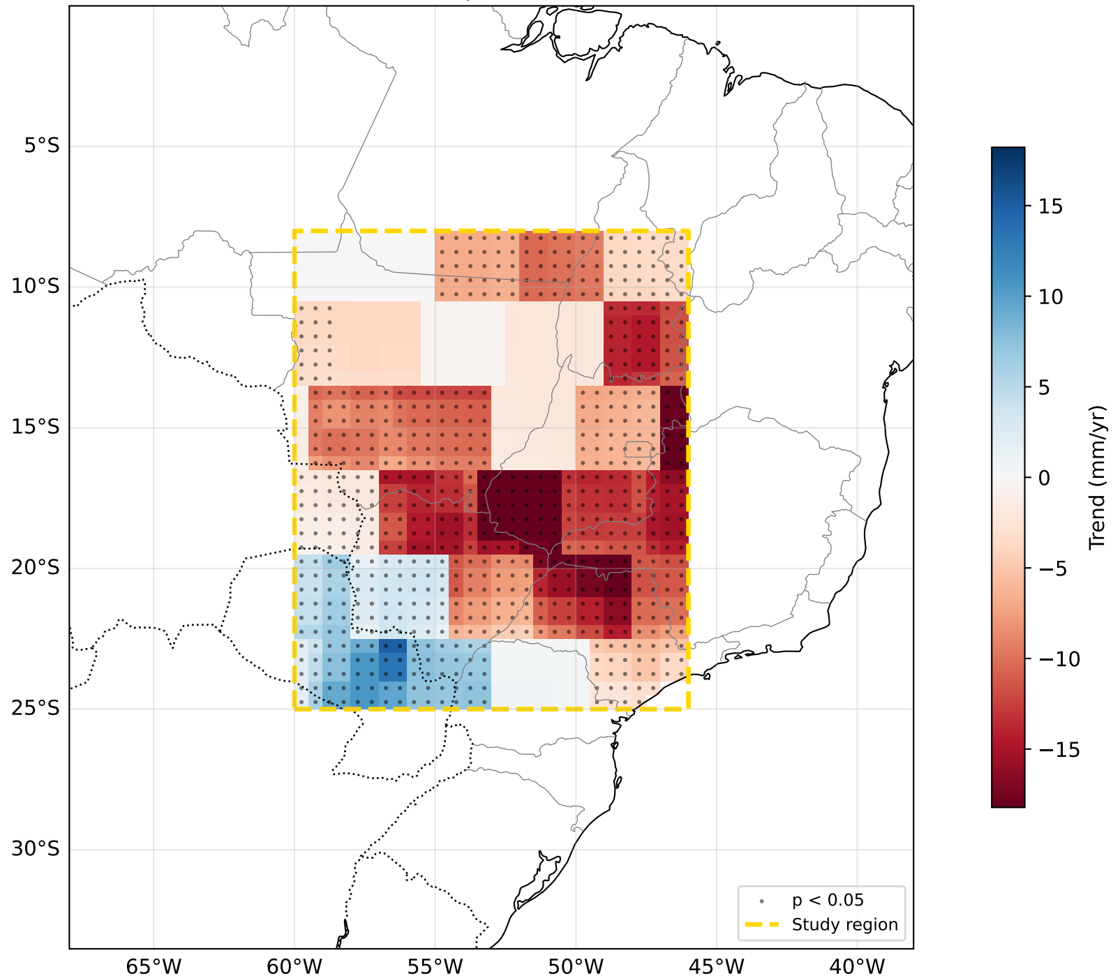
Figure 1 - GRACE TWS Linear Trend in Brazil (2002-2025)
