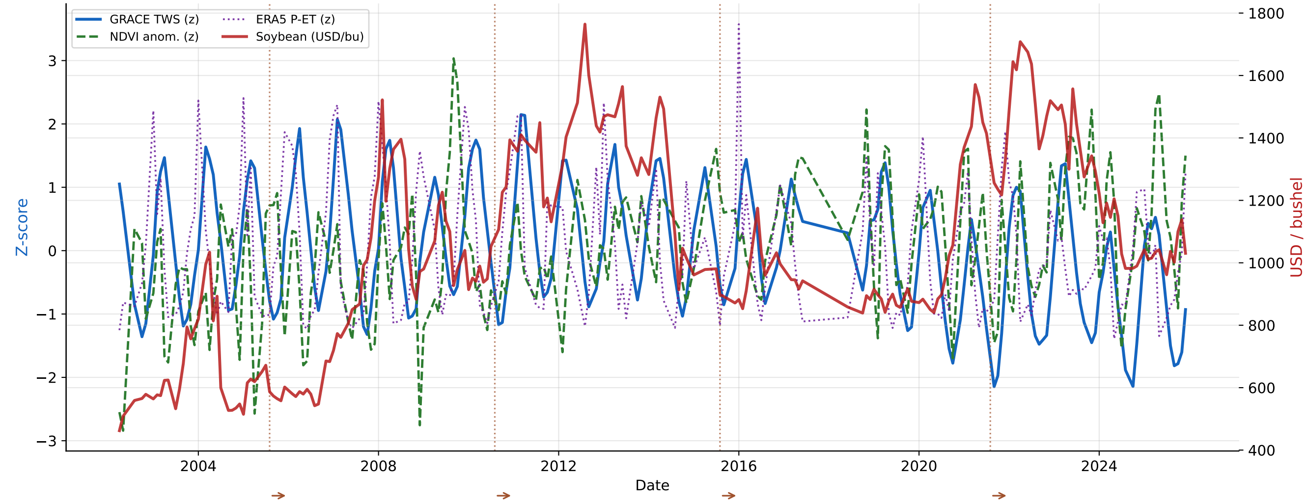
Figure 3 - GRACE TWS \hat{\cdot} NDVI \hat{\cdot} P-ET \hat{\cdot} Soybean Futures Arrows: drought onset \rightarrow market reaction ( \sim 5 months)
