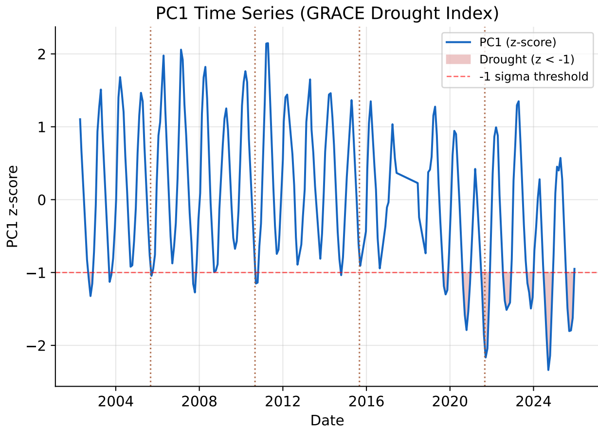
Figure 2 -- EOF Analysis of GRACE TWS (Study Region)
