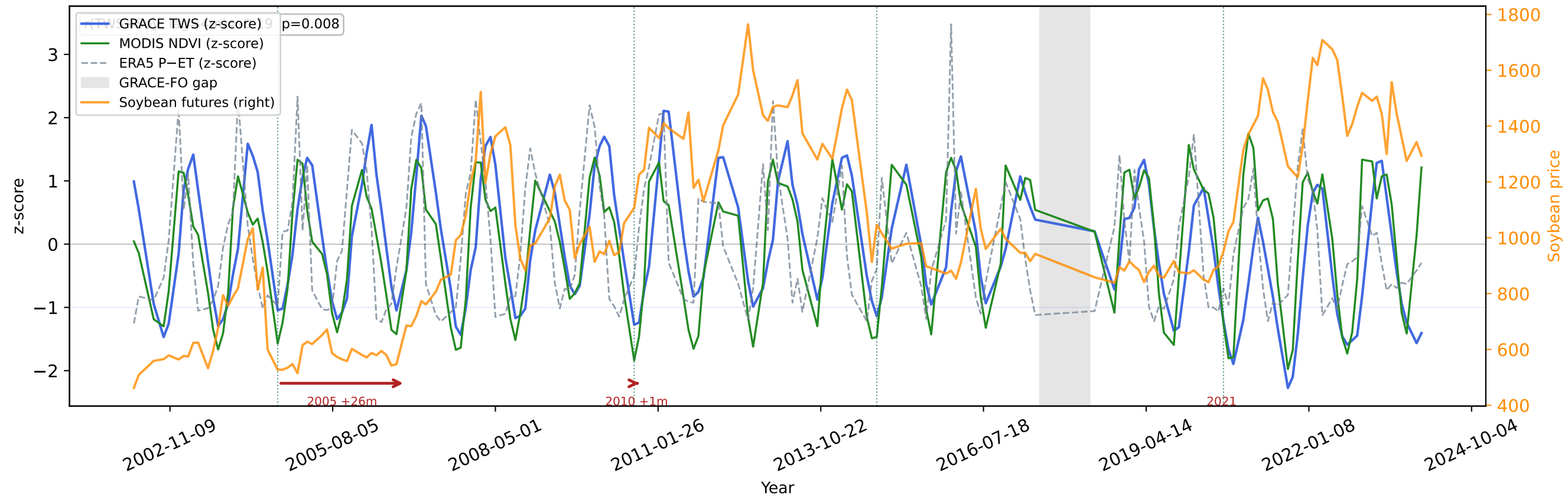
Fig. 3 — GRACE TWS / MODIS NDVI / ERA5 P-ET / Soybean Futures Arrows: drought onset (TWS) → price reaction; vertical lines: TWS→NDVI cascade onset
