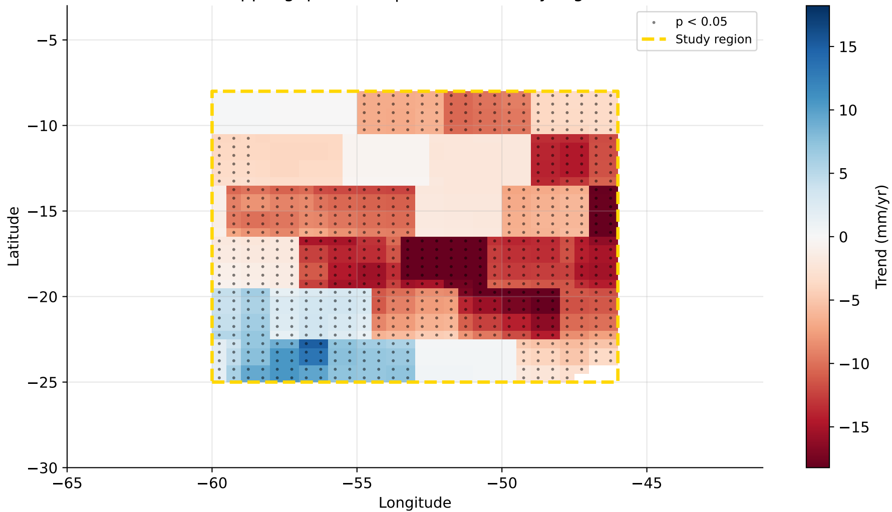
Figure 1 -- GRACE TWS Linear Trend (2002-2025)
