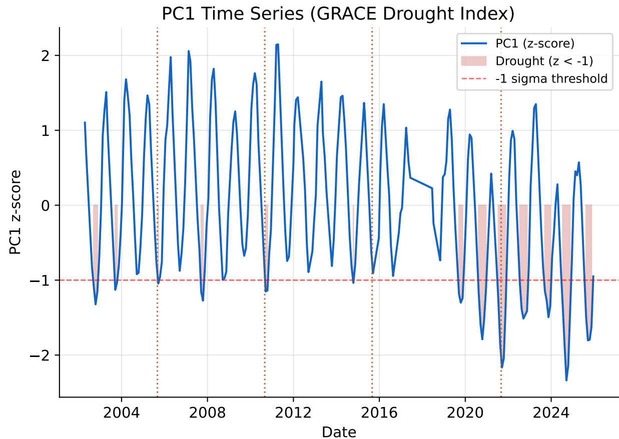
Figure 2 -- EOF Analysis of GRACE TWS (Study Region)
