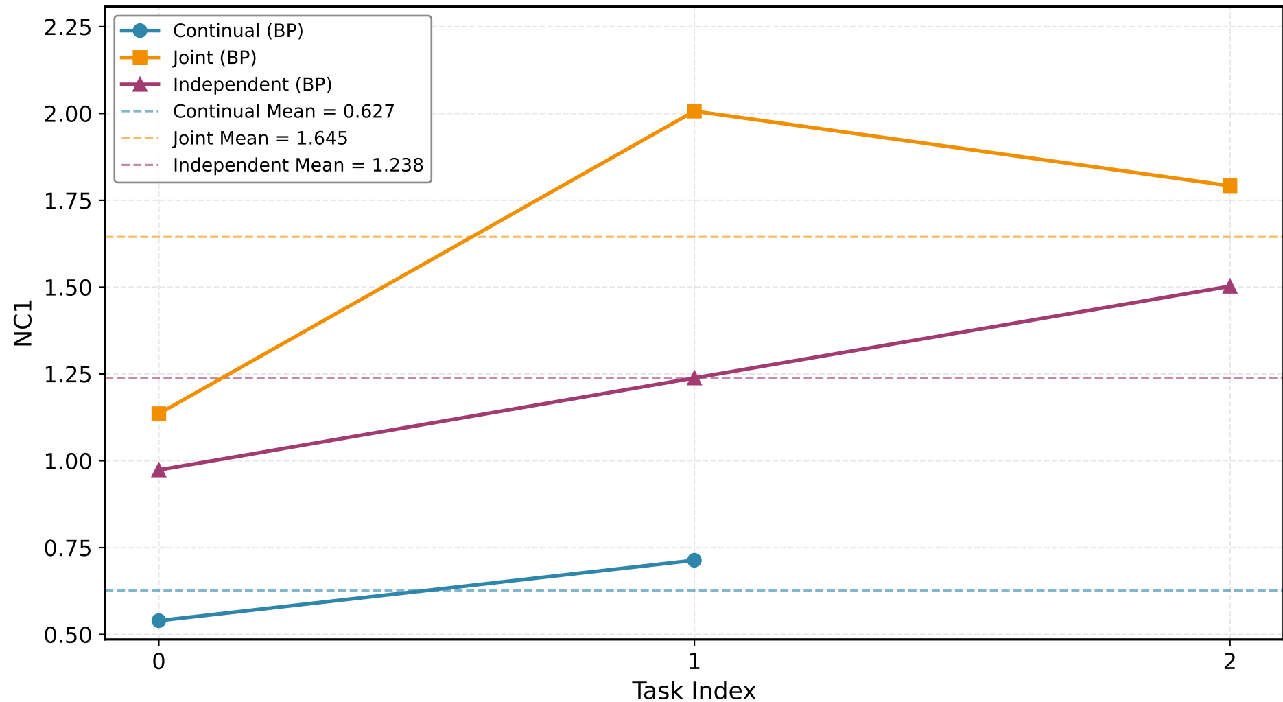
NC1 Across Tasks — BP Algorithm (CIFAR-100, ResNet18)
