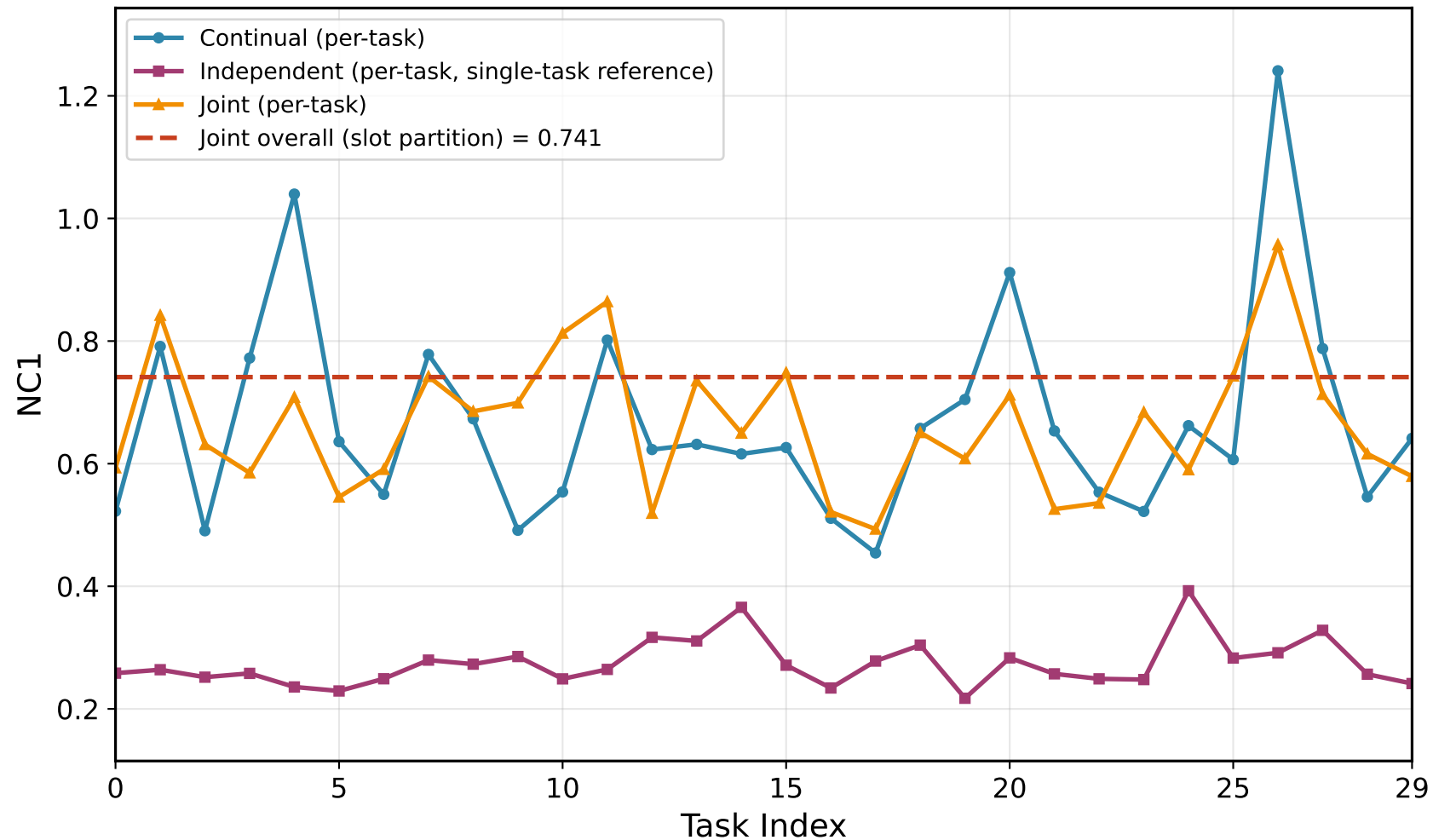
NC1 Evolution Across Tasks (per-task partition) smaller NC1 = stronger collapse
