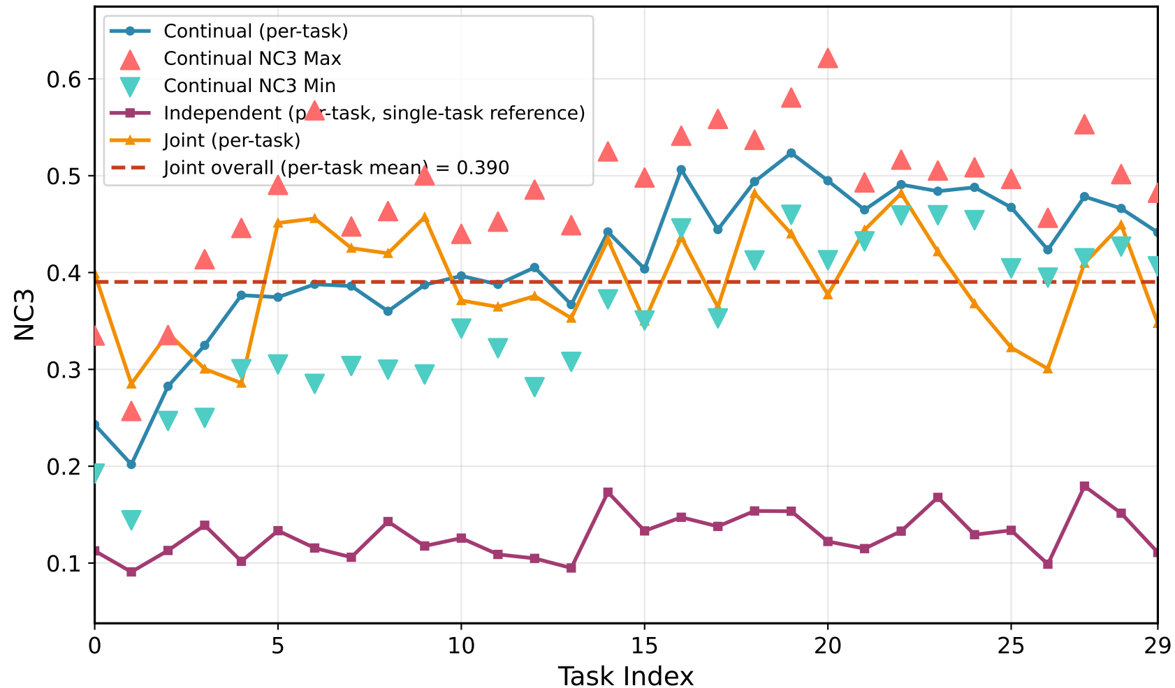
NC3 Evolution Across Tasks (per-task partition) smaller NC3 = stronger self-duality
