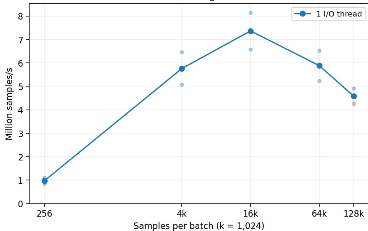
Without training feedback
