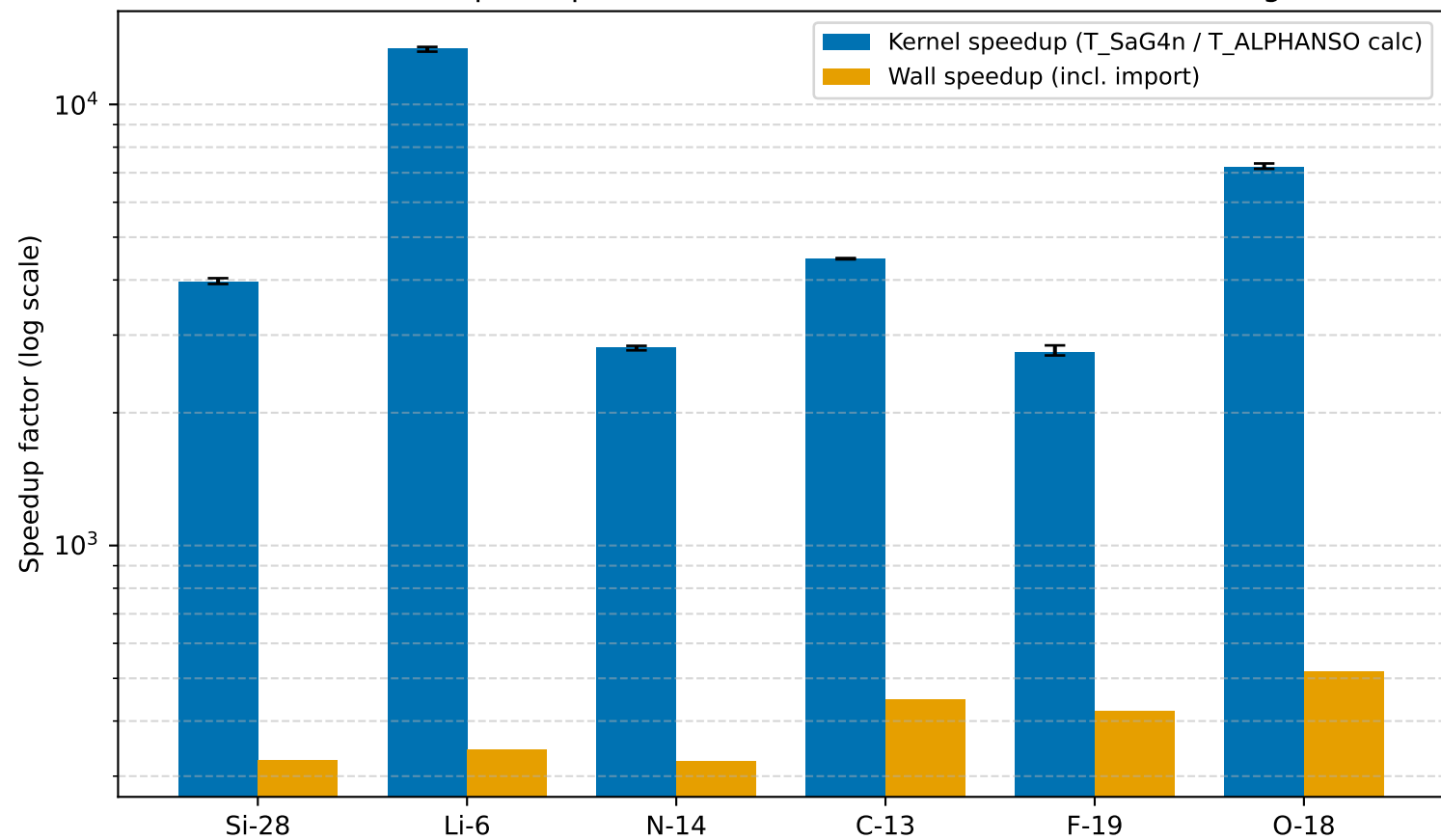
ALPHANSO speedup over SaG4n — Mendoza 2020 Table 2 config
