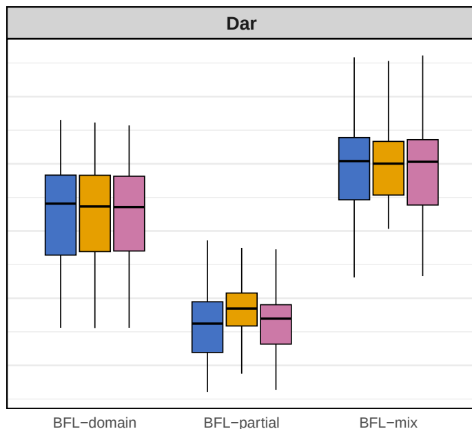
Balanced Accuracy
