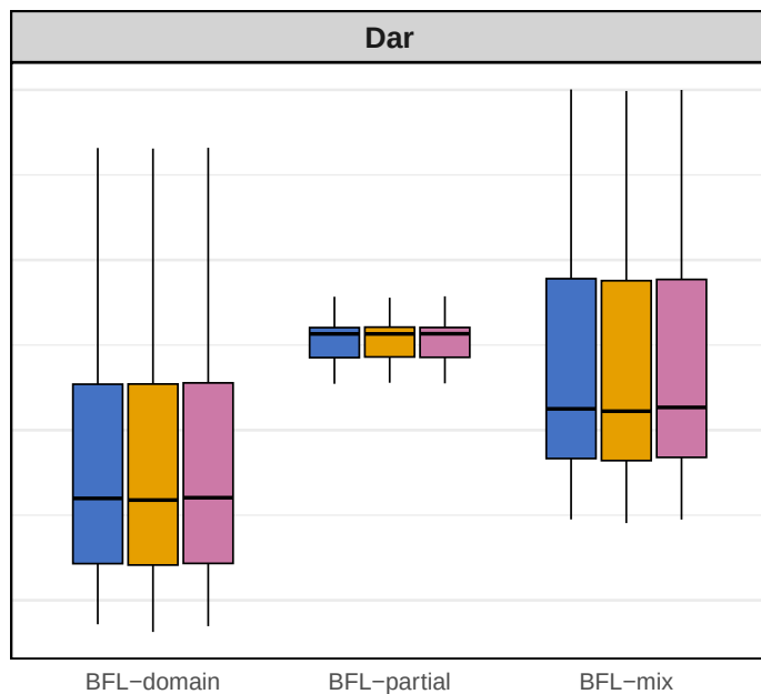
CSMF Accuracy
