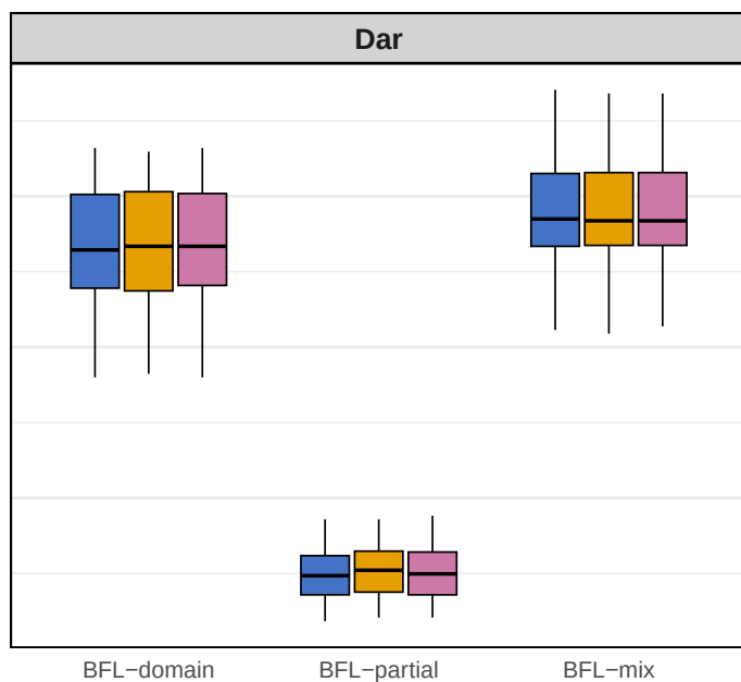
Top-1 Accuracy
