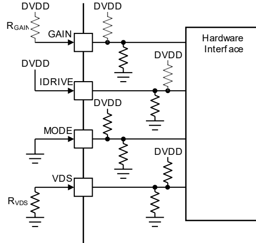
Figure 24. Hardware Interface
