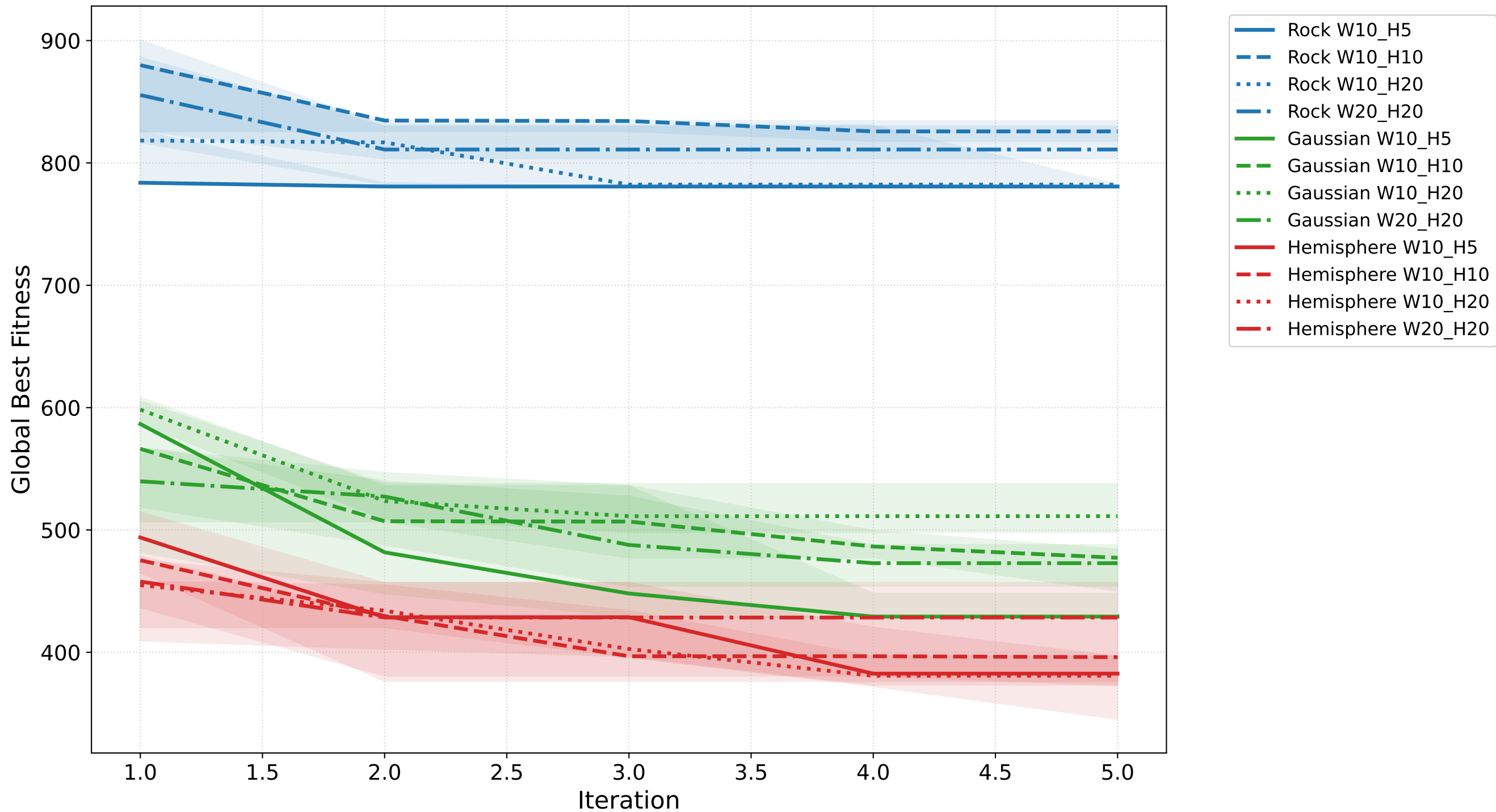
Global Best Fitness Trend Across Terrains and Patch Sizes
