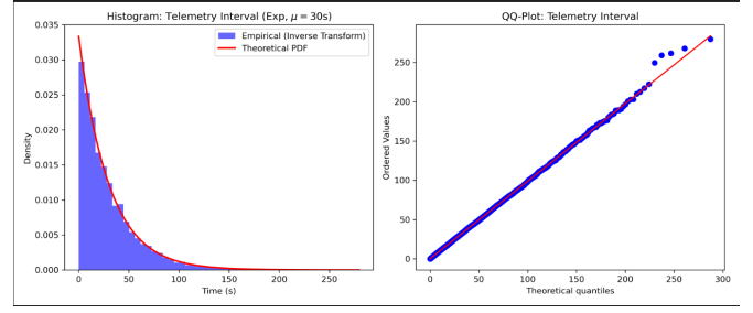
Fig. 4. Input Analysis: Telemetry Interval Distribution and QQ-Plot Fit
