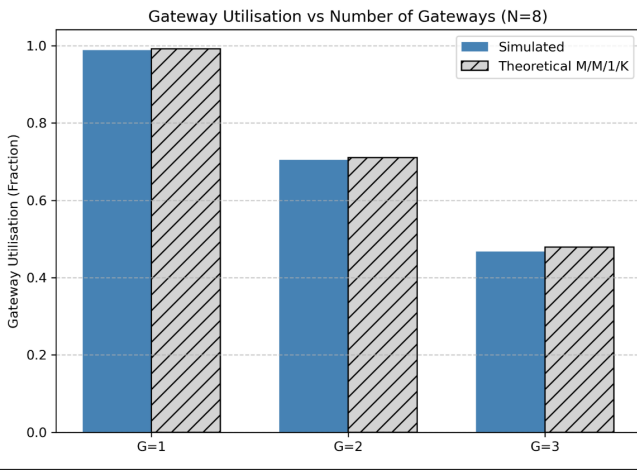
Fig. 8. Gateway Utilisation vs Number of Gateways ( N = 8 )
