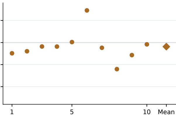
Spectral-state features
