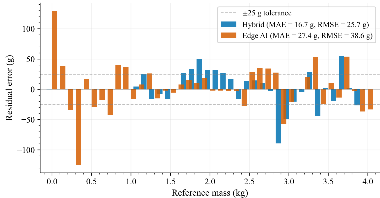
Residual Error at 41 Calibration Reference Points
