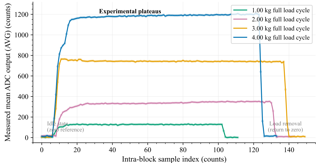
Dynamic Step Response and Return-to-Zero Stability at Multiple Mass Loads
