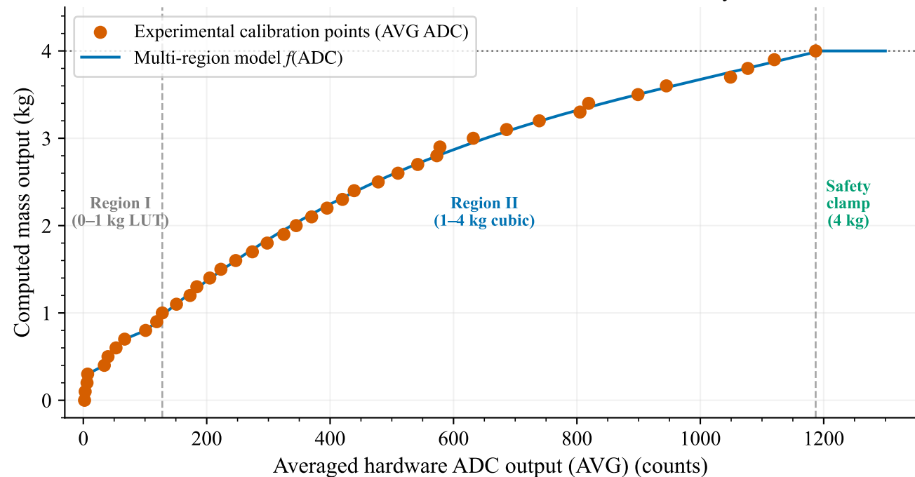
Characteristic Calibration Curve of the Smart Scale System
