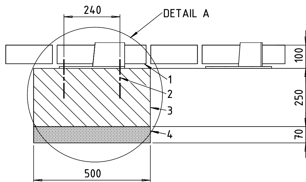
DETAIL A
