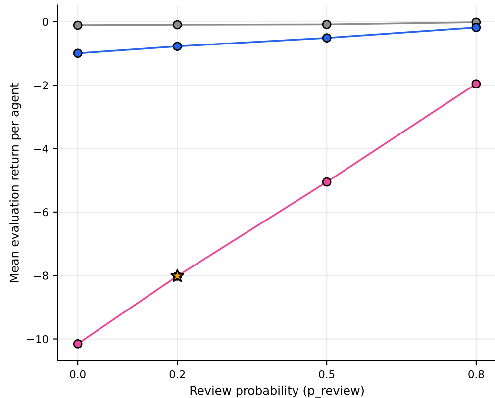
Return sensitivity
