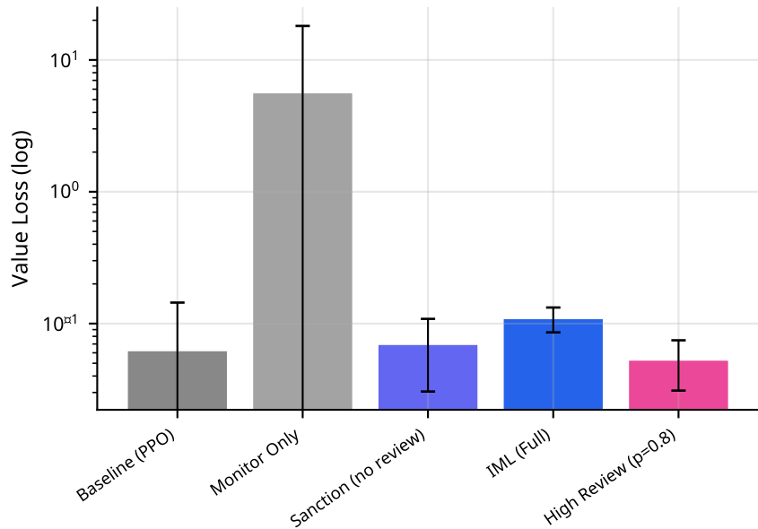
Cleanup — Ablation: Value Loss (log)
