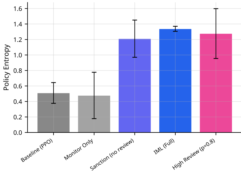
Cleanup — Ablation: Policy Entropy
