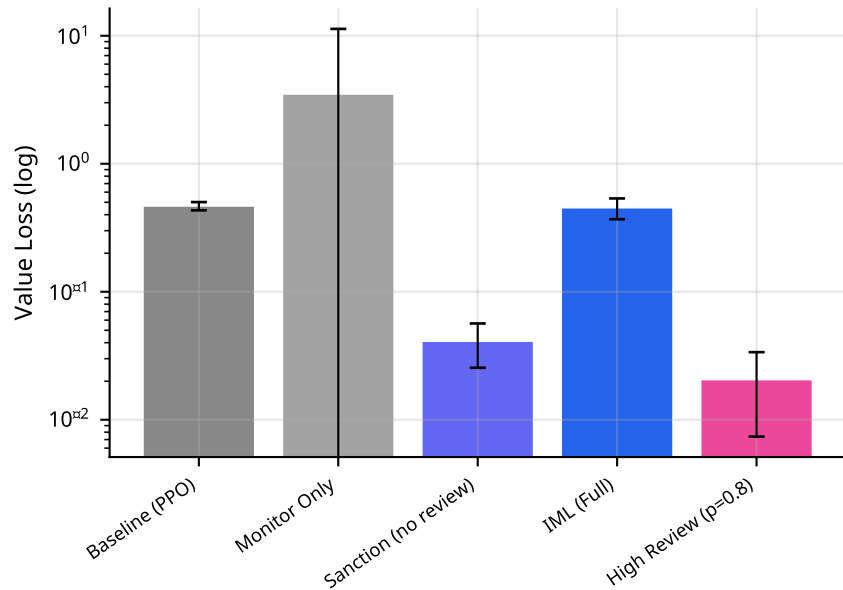
Harvest — Ablation: Value Loss (log)
